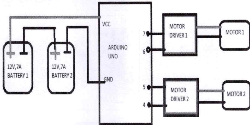
Figure 1: Illustrates the block diagram of the current invention to have an automated wheel chair
